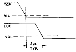
Fig.41 EOC TURN-OFF
